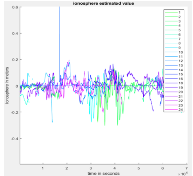
(b) Estimated ionosphere with GLONASS IFCB corrections.
