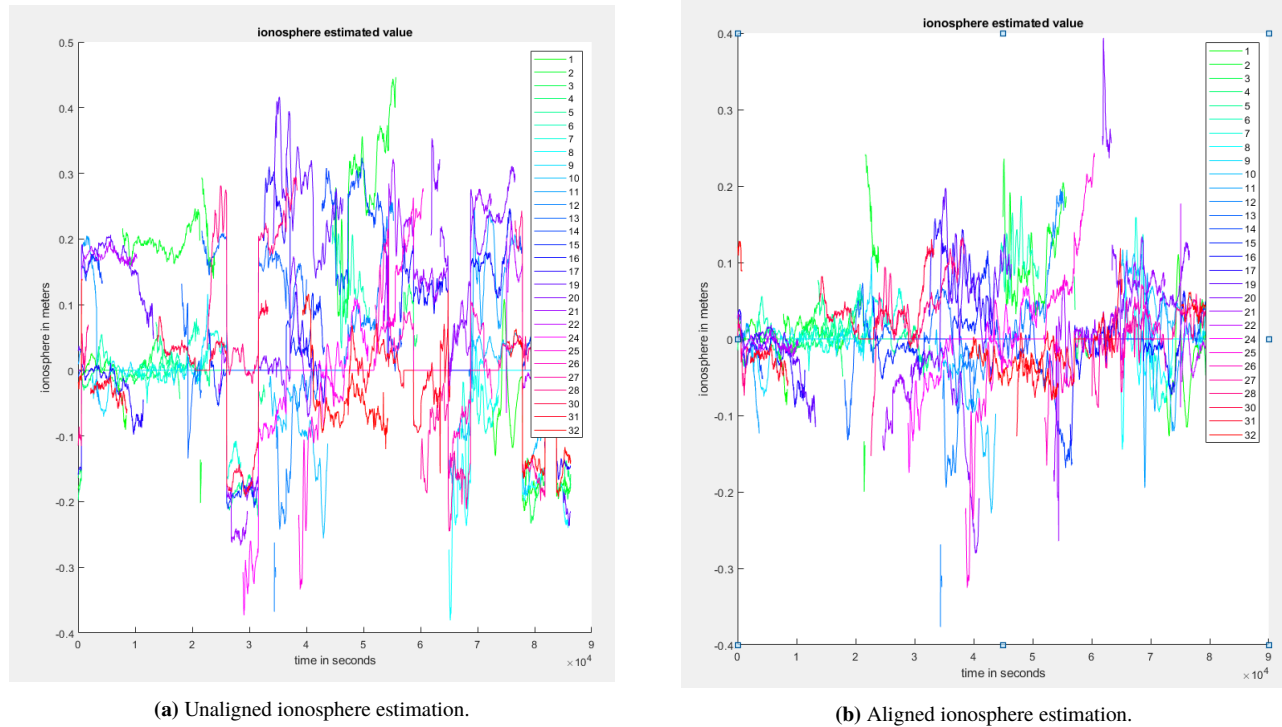
Figure 6: RINEX limitations
