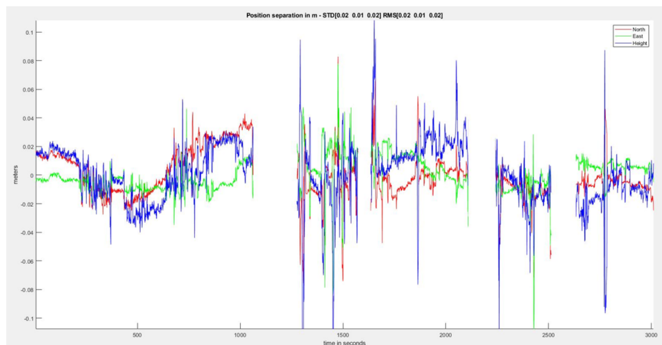
Figure 12: Automotive urban canyon: VBS performance compared to the reference.
