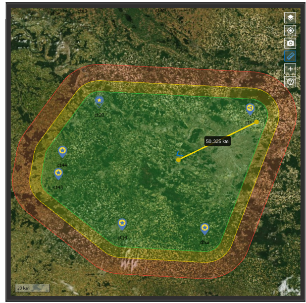
(b) VBS network 2 overview.
