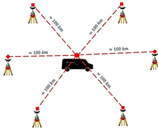
Figure 1: Virtual base station overview.
