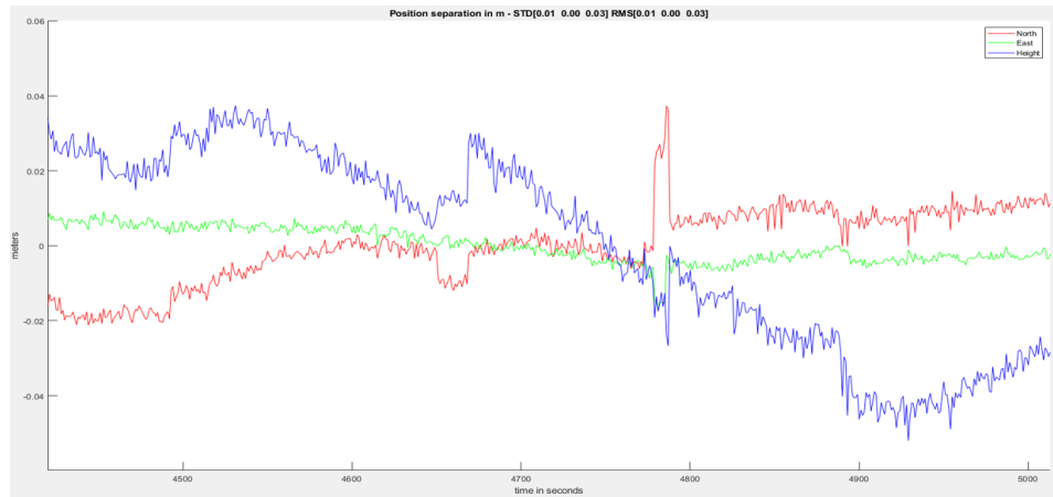
Figure 14: Airplane application: VBS segment 1 performance compared to the reference.
