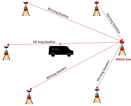
Figure 3: Atmospheric residual estimation.
