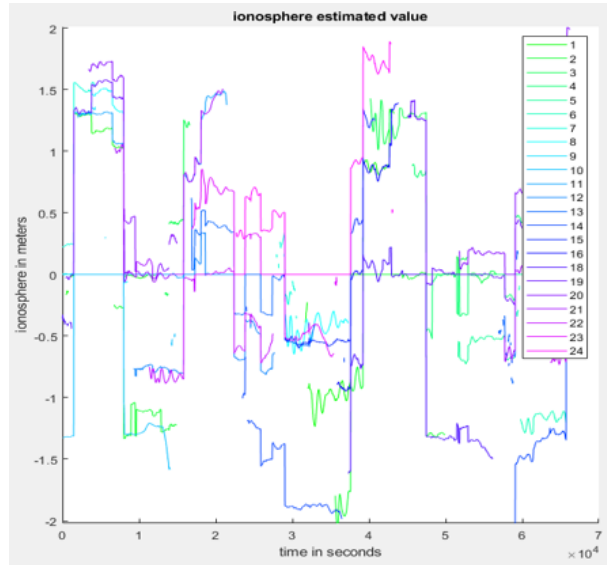
(a) Estimated ionosphere without GLONASS IFCB corrections.
