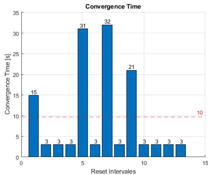
Figure 19: Tightly Coupled INS/GNSS PPP-IF-IAR: Navsight Marine Ambiguity AHRS Resets Convergence Time.
