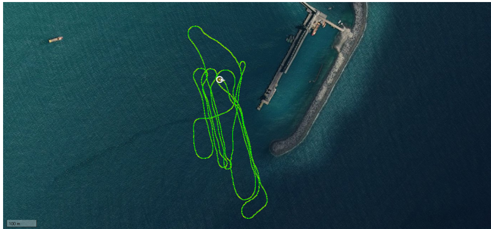
Figure 13: Qinertia Overview of Marine Test Trajectory
