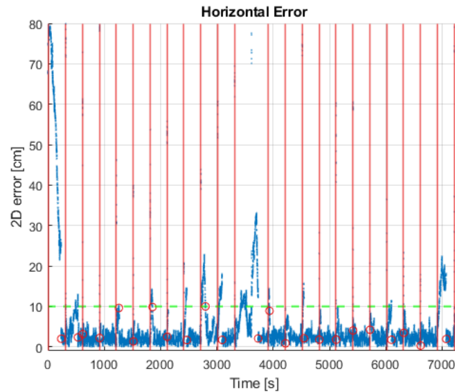
Figure 8: Tightly Coupled INS/GNSS PPP-IF-IAR: Navsight Ekinox Ambiguity AHRS Resets Horizontal Error.
