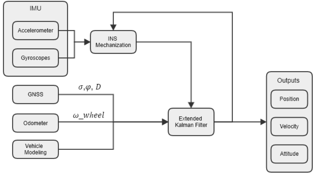
Figure 1: Tightly Coupled INS/GNSS Integration Architecture.
