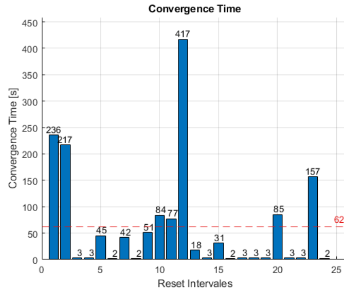
Figure 12: Tightly Coupled INS/GNSS PPP-IF-IAR: Navsight Horizon Ambiguity AHRS Resets Convergence Time.
