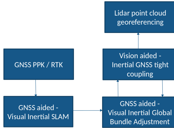
Figure 3: Scheme of the processing workflow in case of difficult GNSS conditions.
