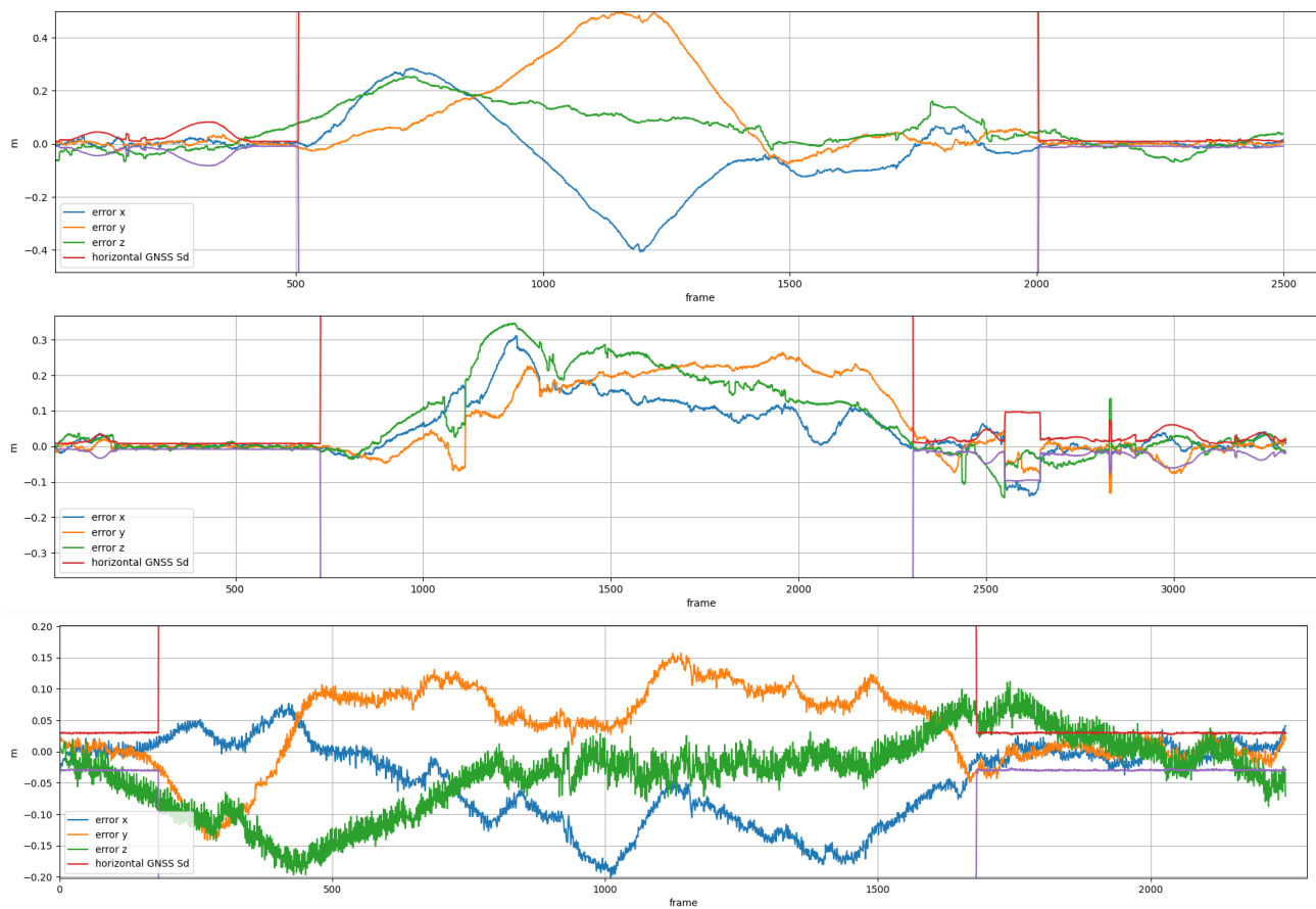
Figure 7: GNSS gaps simulation, From top to bottom: Residential dataset, in town dataset, parking dataset. The GNSS gaps are represented by the horizontal GNSS standard deviation in red and purple on the graphics.
