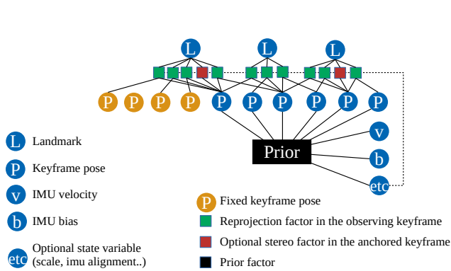
Figure 1: Structure of our SLAM system with 10 keyframes among them 4 are fixed. At each local bundle adjustment the state variables of the landmark (their inverse depth) are substituted using the Schur Complement to obtain a small and dense information matrix.
