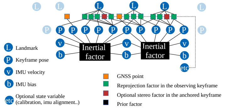
Figure 2: Structure of our global bundle adjustment system. At each global bundle adjustment the state variables of the landmarks are substituted using the Schur Complement to form a big and sparse information matrix. Resolution is done using a conjugate gradient with block-diagonal preconditioning. In order to reduce the problem size we use only 1 inertial state every 5 visual states, assuming that the inertial preintegration does not drift too much after 5 images.
