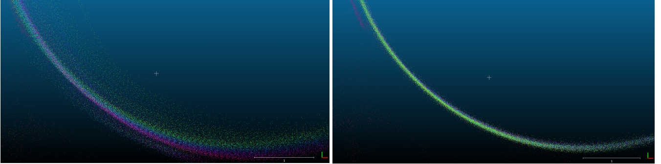
Figure 8: Point cloud of a water tank before calibration (left) and after calibration (right). Units in meters. The calibration parameters converged within 3 iterations. At the first iteration 2817 planes were used and at the last iteration 4965 plane were used. The boresight angle was corrected by 3^\circ and the lever arm by 20cm. The point cloud used for calibration is plotted at the beginning of the paper.
