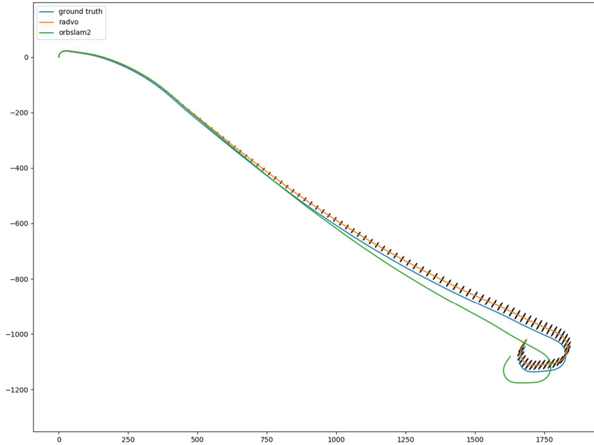
Figure 7: Results on KITTI dataset 01 (orange : ours , blue :ground truth, green : ORB-SLAM2 , black : uncertainty ellipses)
