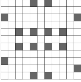
Figure 1: position of the pixels used for the descriptor. There are 16 pixels distributed in a sparse manner in a 11x11 window around the feature center. The descriptor is the concatenation of the intensity of the smoothed x gradient and y gradient (ie. sobel transform) at these pixel positions.
