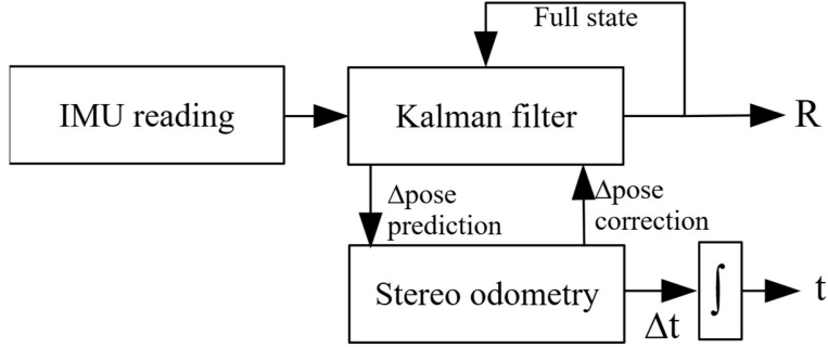
Figure 5: IMU and Stereo odometry coupling.
