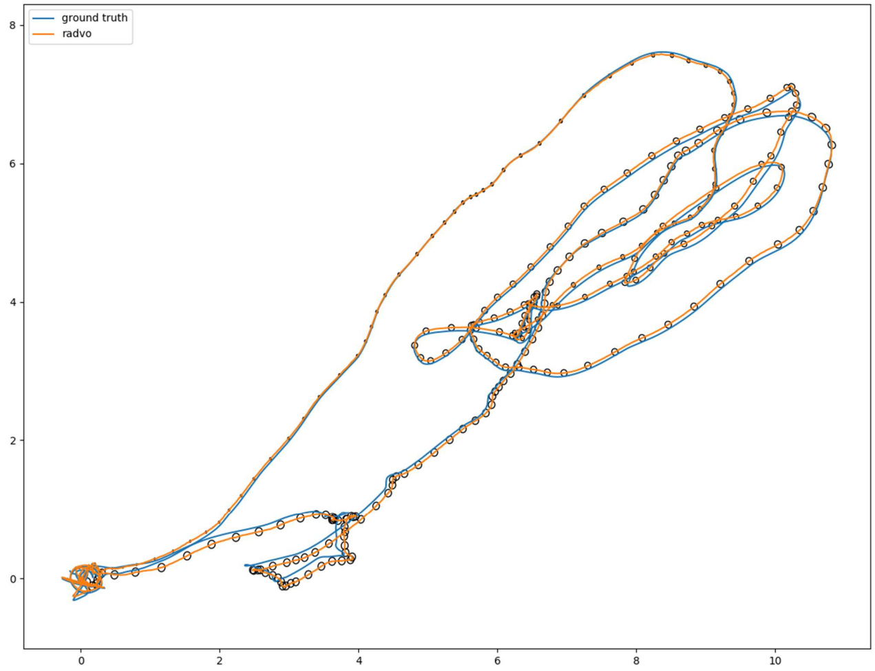
Figure 8: Results on MH_01 dataset (orange : ours , blue :ground truth, black : uncertainty ellipses)
