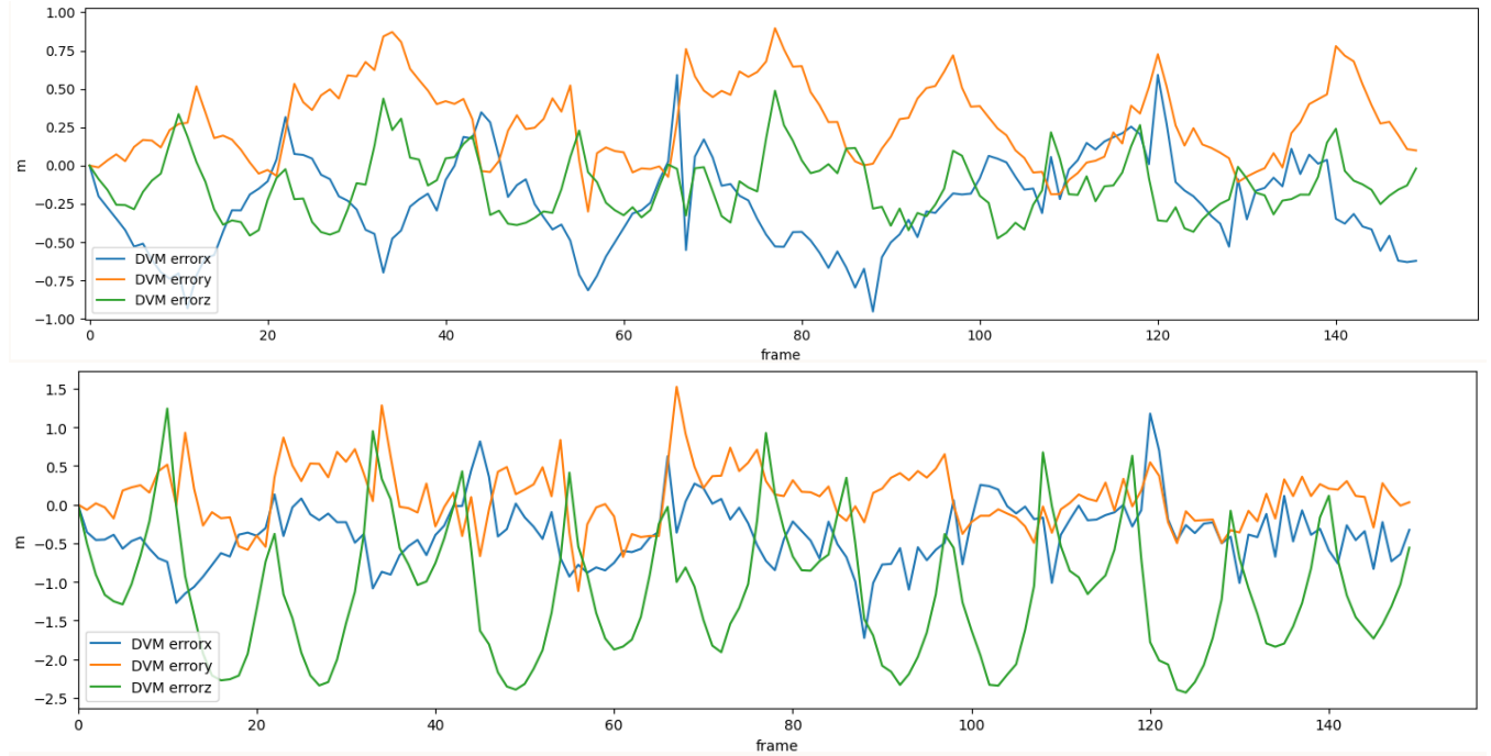
Figure 6: Difference between GNSS and our results after global bundle adjustment. Top: reusing the camera distortion parameter estimated from a GNSS aided run. Bottom: estimating the camera distortion without prior. The unaided calibration run exhibit higher error on x and y and a particular error on z which is characteristic of an erroneous curvature of the global trajectory of the UAV. This particular error can be explained by the ambiguity between the soil curvature and the camera radial distortion.
